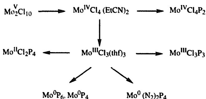
Scheme 1. P=tertiary phosphine \text{PR}_3 ; the nature of R can determine the stoichiometry and isomeric form of the product. thf=tetrahydrofuran.
