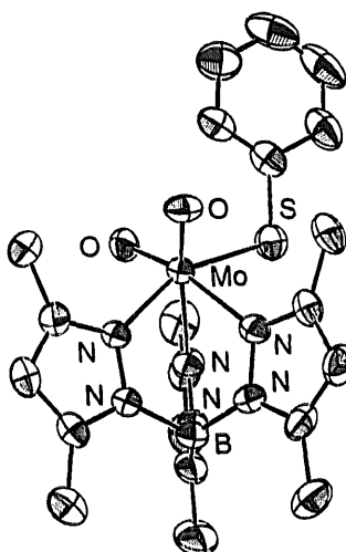
Fig. 1. Molecular Structure of L^c\text{Mo}^{\text{VI}}\text{O}_2(\text{SPh}) .
